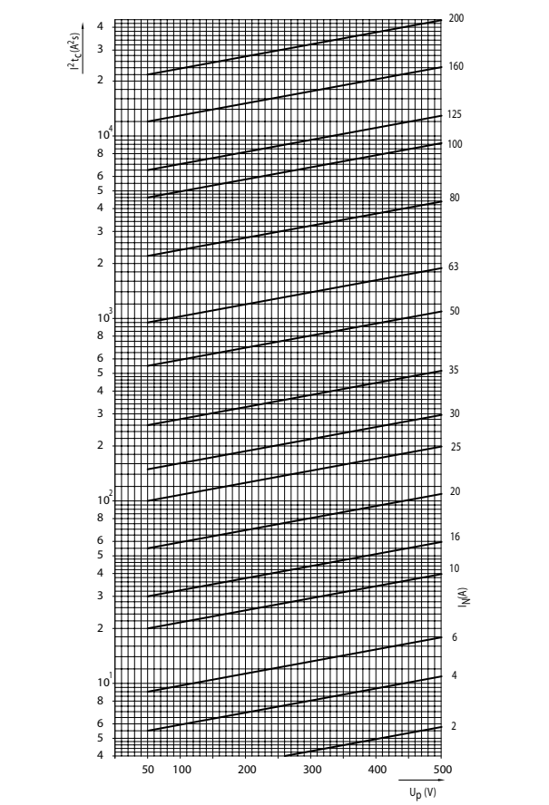
Operating Joule Integral (I 2 t) for Ultra Quick DI, DII, DIII, DIV, DV
